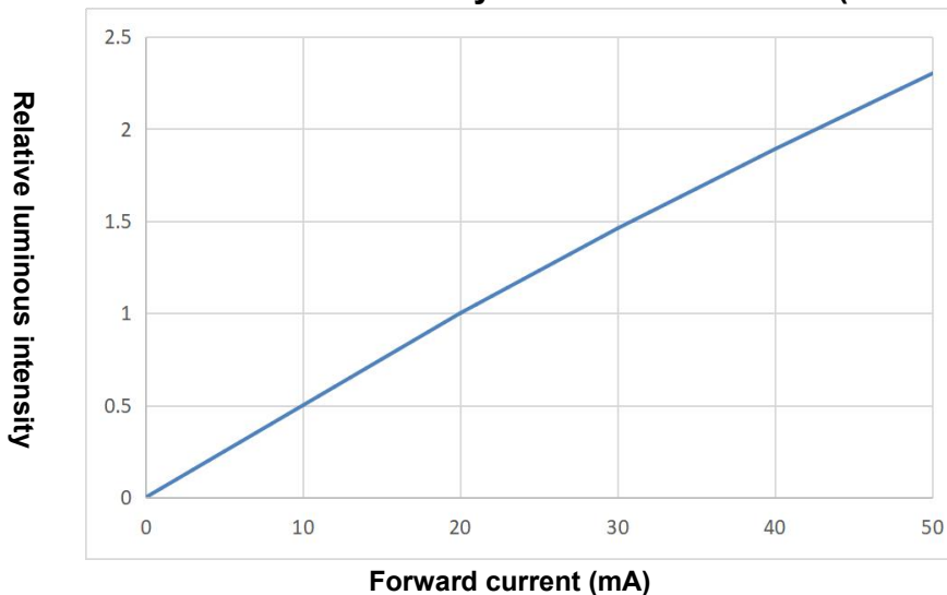
Relative luminous intensity VS. Forward current (Ta=25°C)
