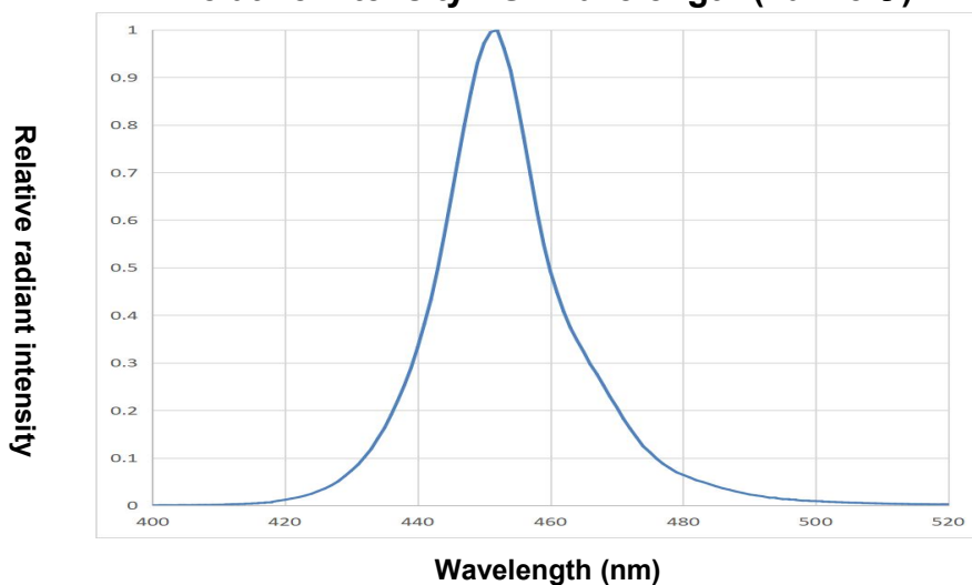
Relative intensity VS. Wavelength (Ta=25°C)
