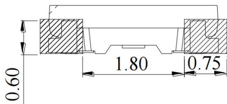
Recommended soldering pad design
