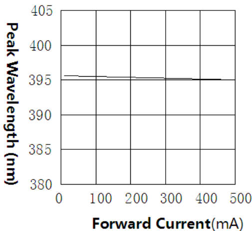
正向电流与峰值波长关系曲线图 Forward Current Vs. Peak Wavelength
