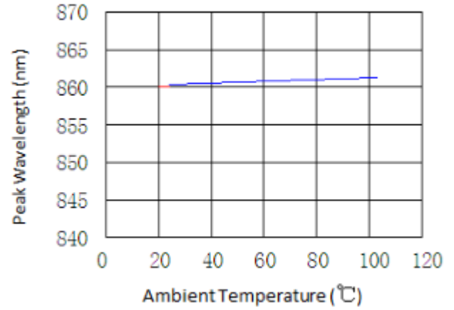
Peak Wavelength VS Ambient Temperature
