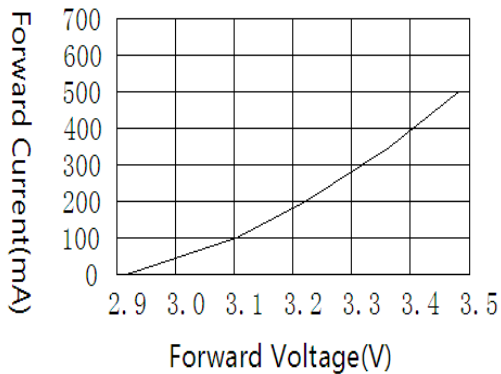
电压与电流关系曲线图 Forward Voltage VS Forward Current
